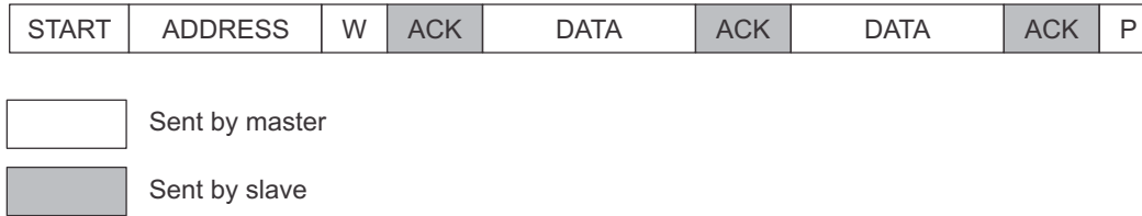
Figure 3-2. Byte Level ACK
