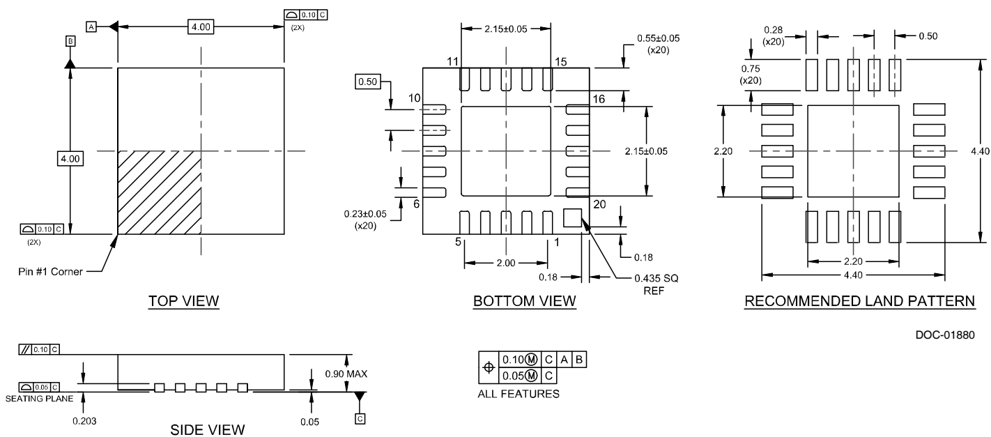
Figure 27. Package Drawing 20-lead 4 × 4 mm QFN
