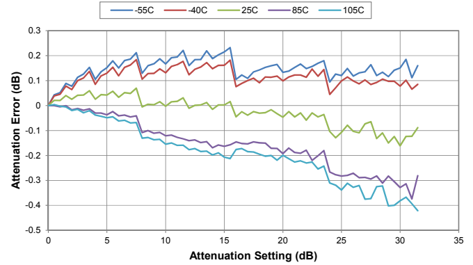
Figure 20. Attenuation Error @ 100 MHz vs Temperature
