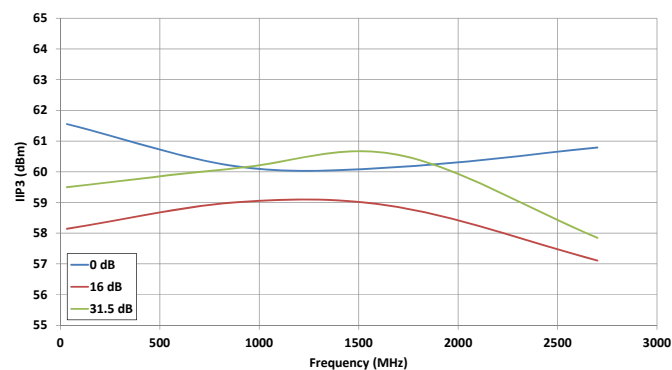
Figure 18. IIP3 vs Frequency
