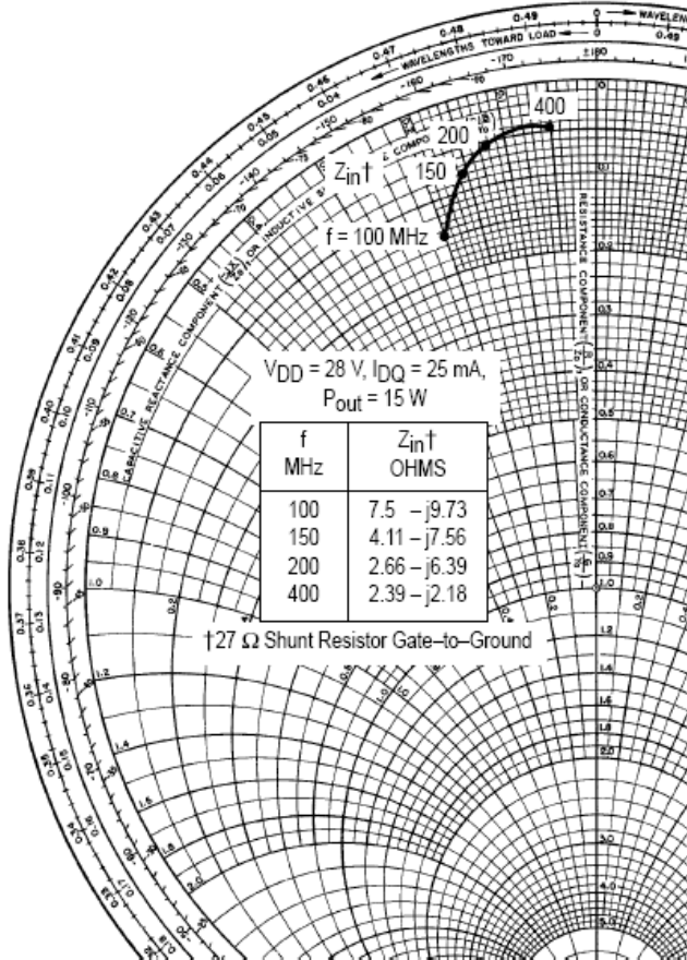
Figure 16. Large-Signal Series Equivalent Input Impedance, Z_{in}\uparrow
