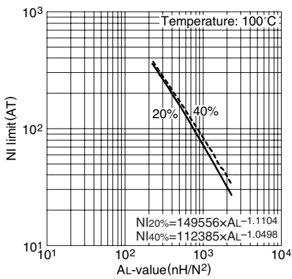
NI limit vs. AL-value for PC40EE60 gapped core (Typical)
