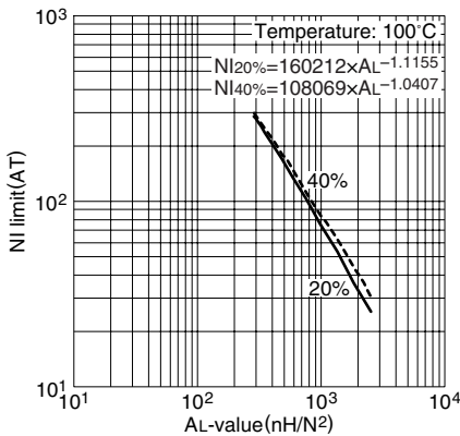
NI limit vs. AL-value for PC40EI60 gapped core (Typical)
