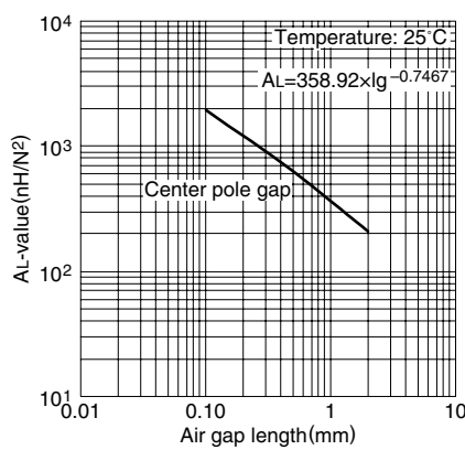
AL-value vs. Air gap length for PC40EE60 core (Typical)
