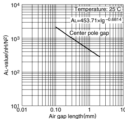
AL-value vs. Air gap length for PC40EI60 core (Typical)
