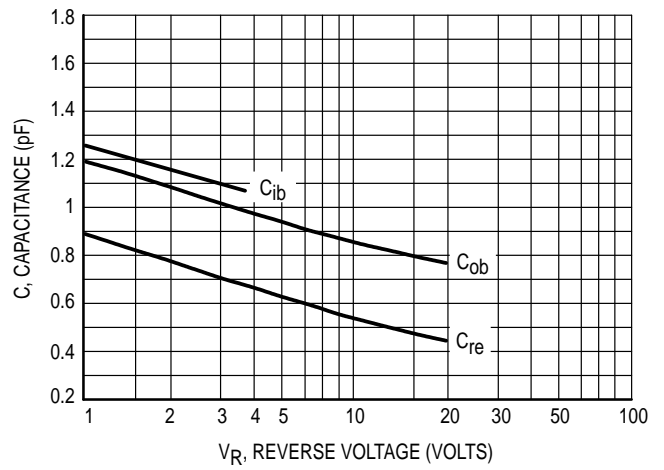
Figure 4. Capacitances
