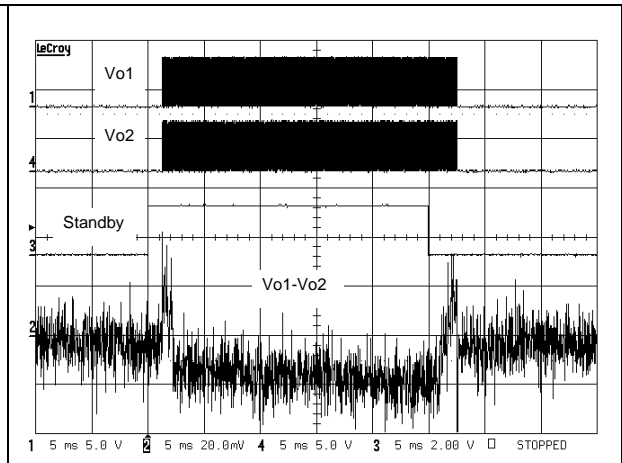
Figure 55. Startup & shutdown time V_{CC} = 5V , G = 6\text{ dB} , C_{in} = 1\text{ }\mu\text{F} (5 ms/div)
