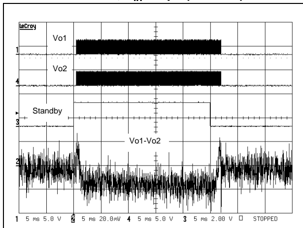
Figure 56. Startup & shutdown time V_{CC} = 3V , G = 6\text{ dB} , C_{in} = 1\text{ }\mu\text{F} (5 ms/div)
