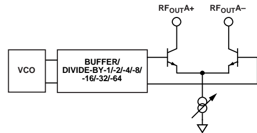
Figure 22. Output Stage
