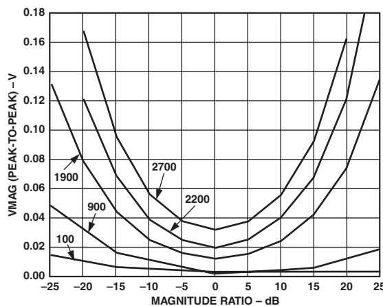
TPC 24. VMAG Peak-to-Peak Output Induced by Sweeping Phase Difference through 360 Degrees vs. Magnitude Ratio, Frequencies 100 MHz, 900 MHz, 1900 MHz, 2200 MHz, and 2700 MHz
